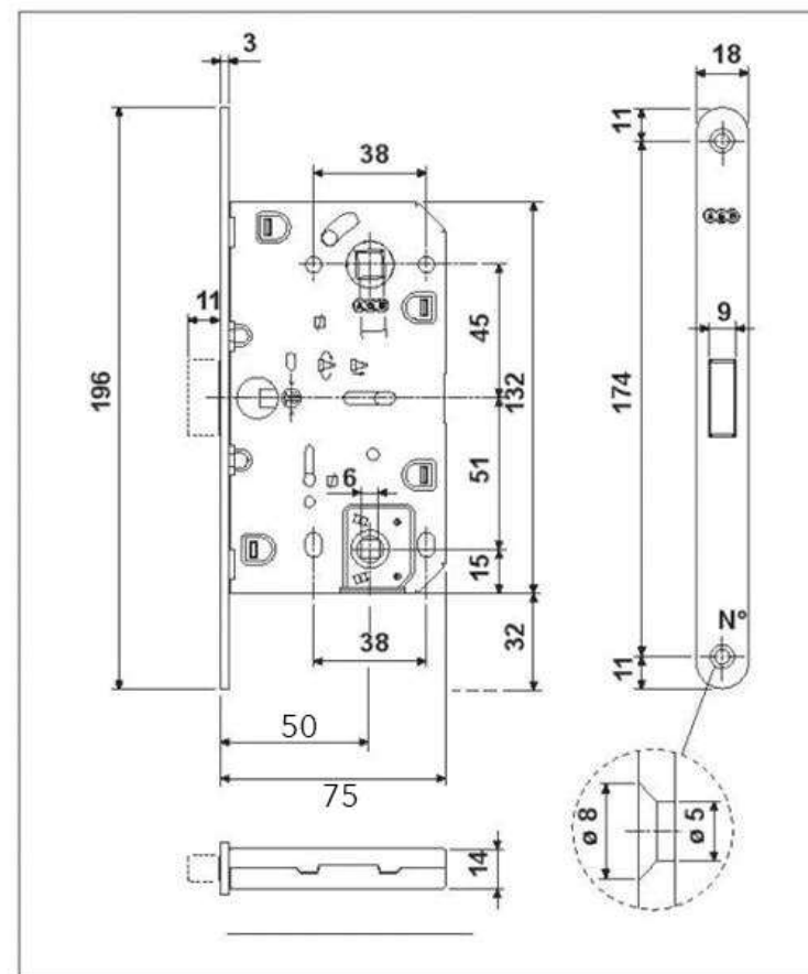
Product Dimensions
