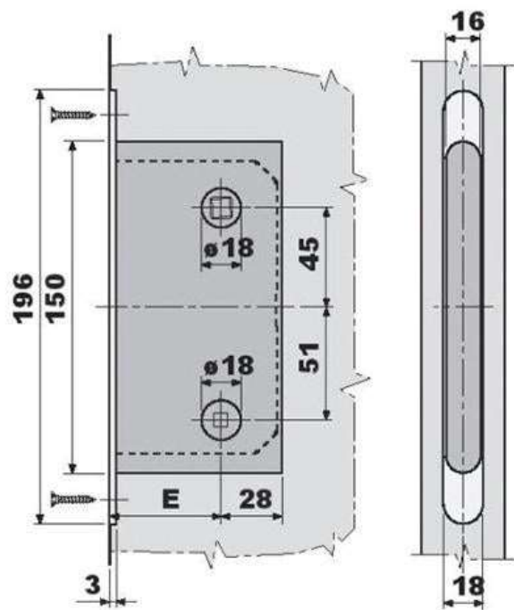
Drilling Diagram
